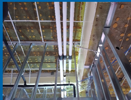
Installation of Overhead Pipes and Pipe Insulation in Building 2010
